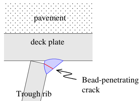
Fig. 2. Bead-penetrating crack
