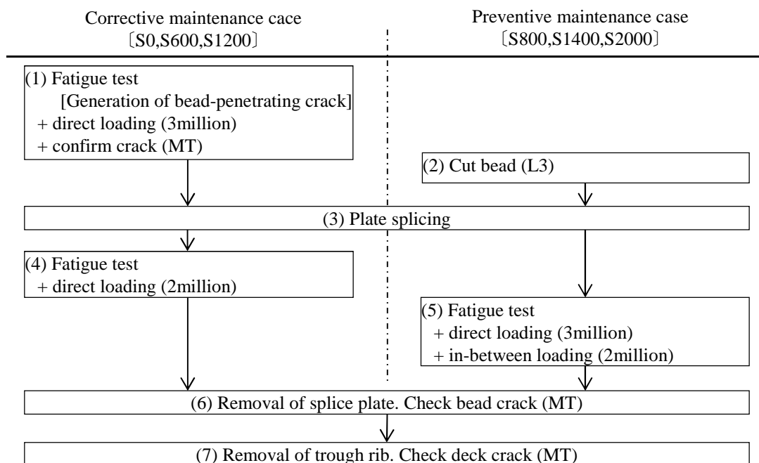
Fig. 8. Test flow of test model 2
