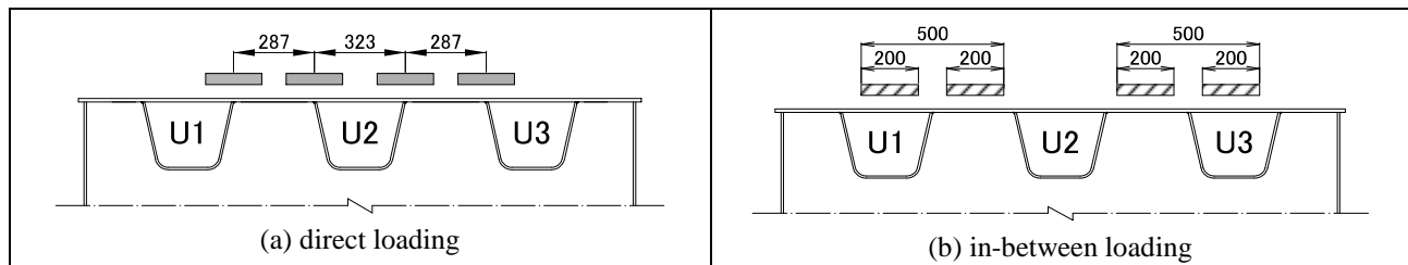
Fig. 5. Loading pattern
