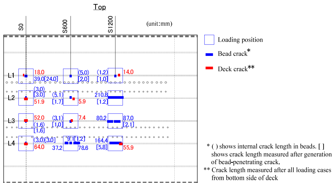
Fig. 11. Crack distribution (after fatigue test)
