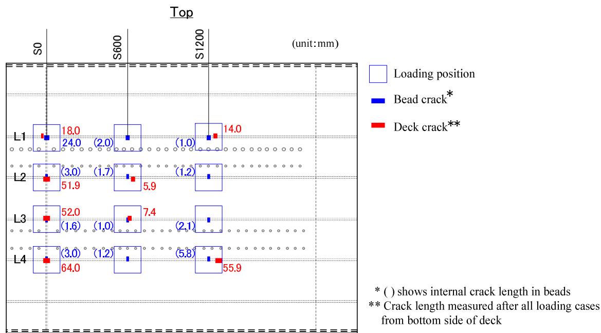
Fig. 10. Crack distribution (after generation of bead-penetrating crack)
