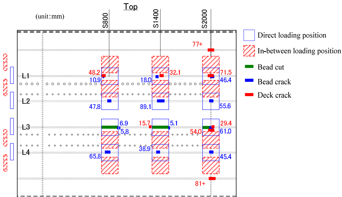
Fig. 12. Crack distribution (after all loading)
